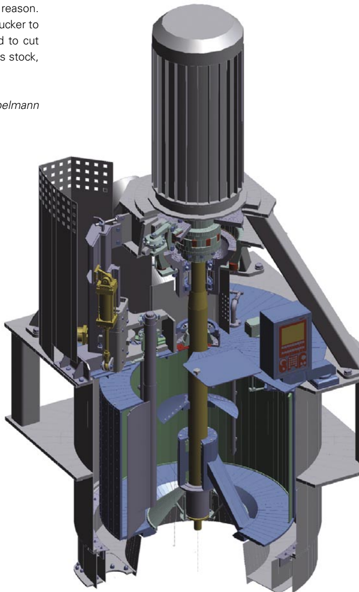
Batch centrifugal of the 'B' series
